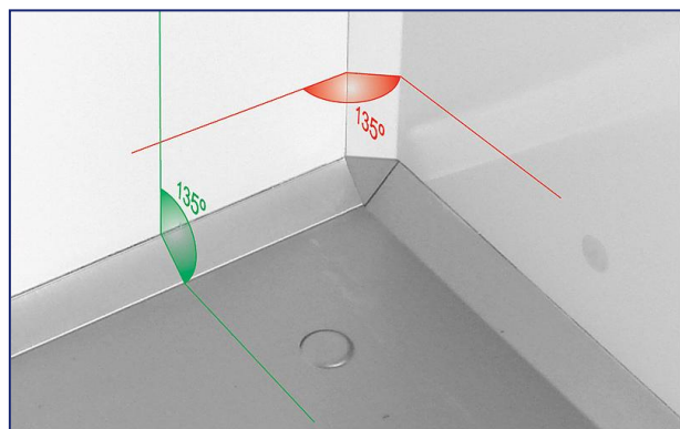
Preformed sanitary corners (135° wide angle)
