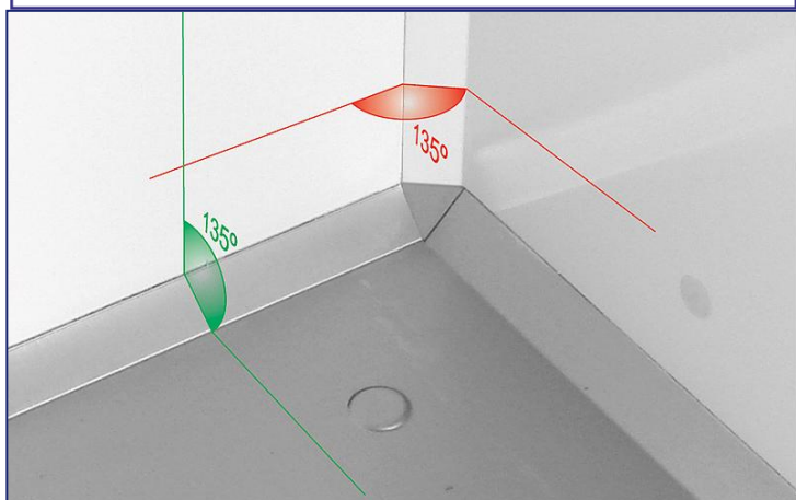
Preformed sanitary corners (135° wide angle)
